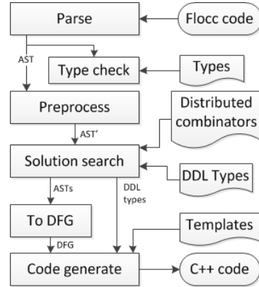
Fig. 13 Compiler architecture
