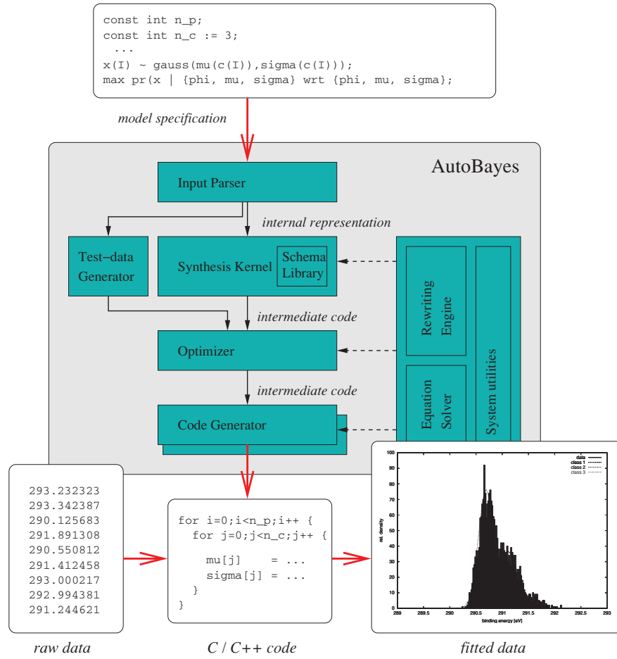
Fig. 4. System architecture of AUTOBAYES.
