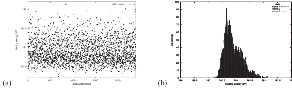
Fig. 2. (a) Artificial input data for the mixture of Gaussians example: 2400 data points in the range [290.2, 292.2]. Each point belongs to one of three classes which are Gaussian distributed with \mu_1 = 290.7, \sigma_1 = 0.15 , \mu_2 = 291.13, \sigma_2 = 0.18 , and \mu_3 = 291.55, \sigma_3 = 0.21 . The relative frequencies \phi for the points belonging to the classes are 61%, 33%, and 6%, respectively. (b) Histogram (spectrum) of the artificial test data from (a) and Gaussian distributions which are obtained as the result of the synthesized data analysis program.
